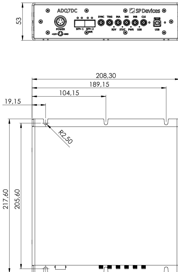
Figure 5: Box drawing for –USB interface options.
