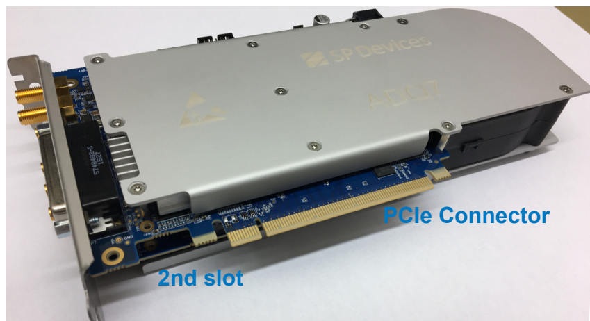
Figure 9: ADQ7–PCIE extends to the left of the connector.
