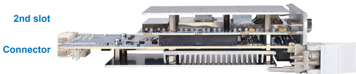
Figure 6: ADQ7–PXIE extends to the left of the connector. Bottom view with the handle to the right.
