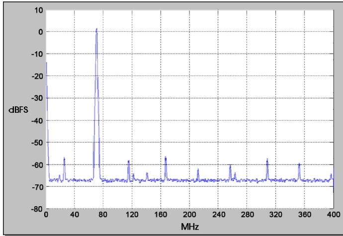
f_{out} = 70 \text{ MHz} , f_s = 800 \text{ MHz} , Interpolation = 4, Internal Clock
