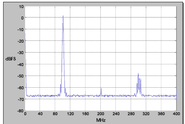
f_{out} = 100 \text{ MHz} , f_s = 800 \text{ MHz} , Interpolation = 4, Internal Clock
